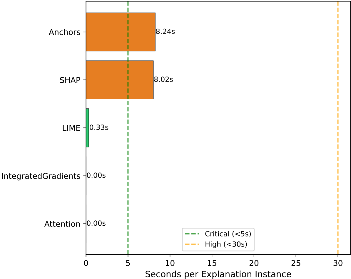
XAI Method — Explanation Time (SOC Triage Windows)
